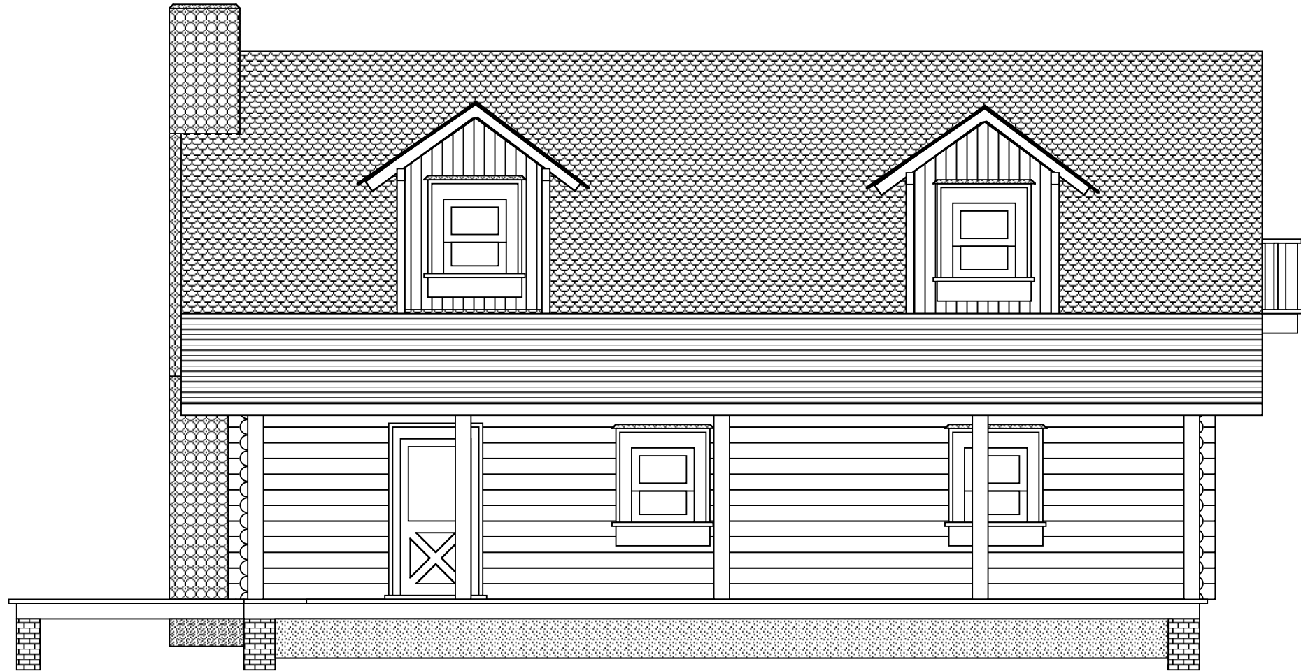
REAR ELEVATION
